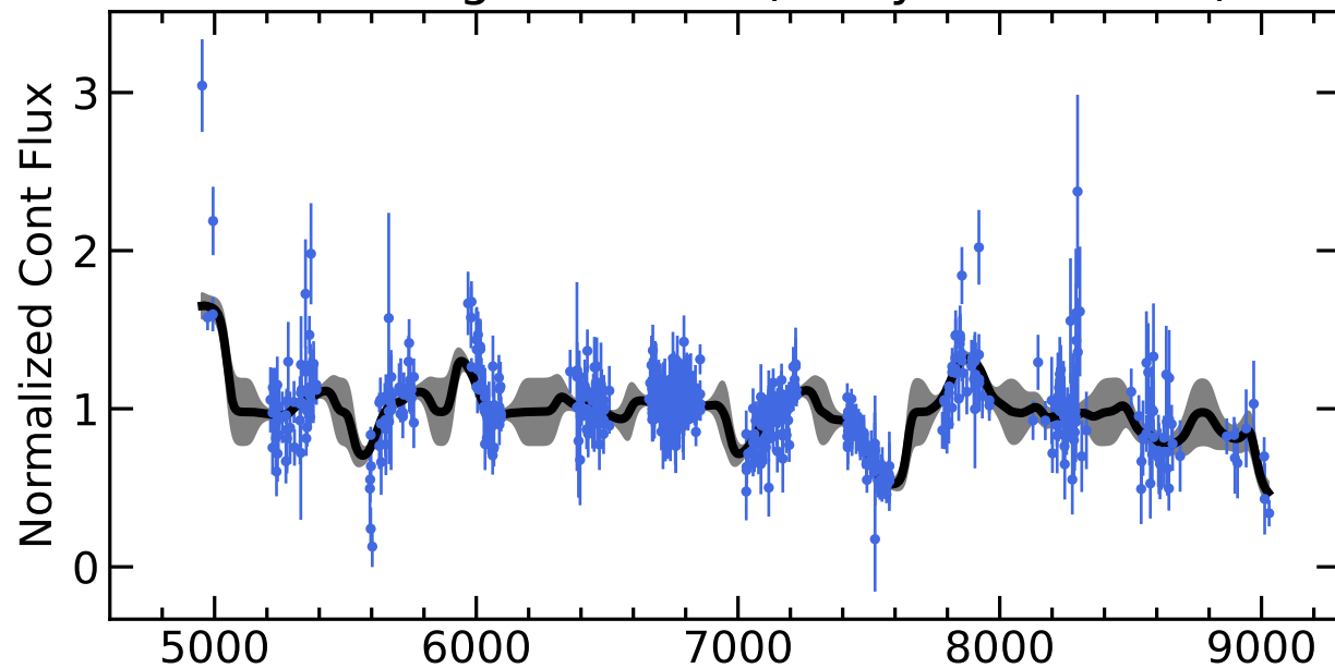
RM791 Light Curves (w/ PyROA model)
