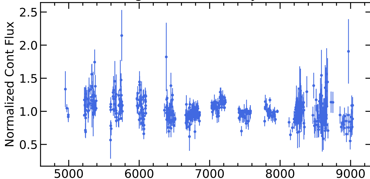
RM792 Light Curves (w/ PyROA model)
