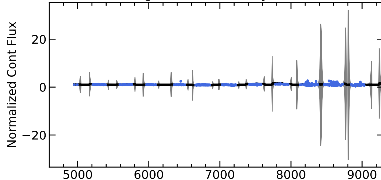
RM794 Light Curves (w/ PyROA model)
