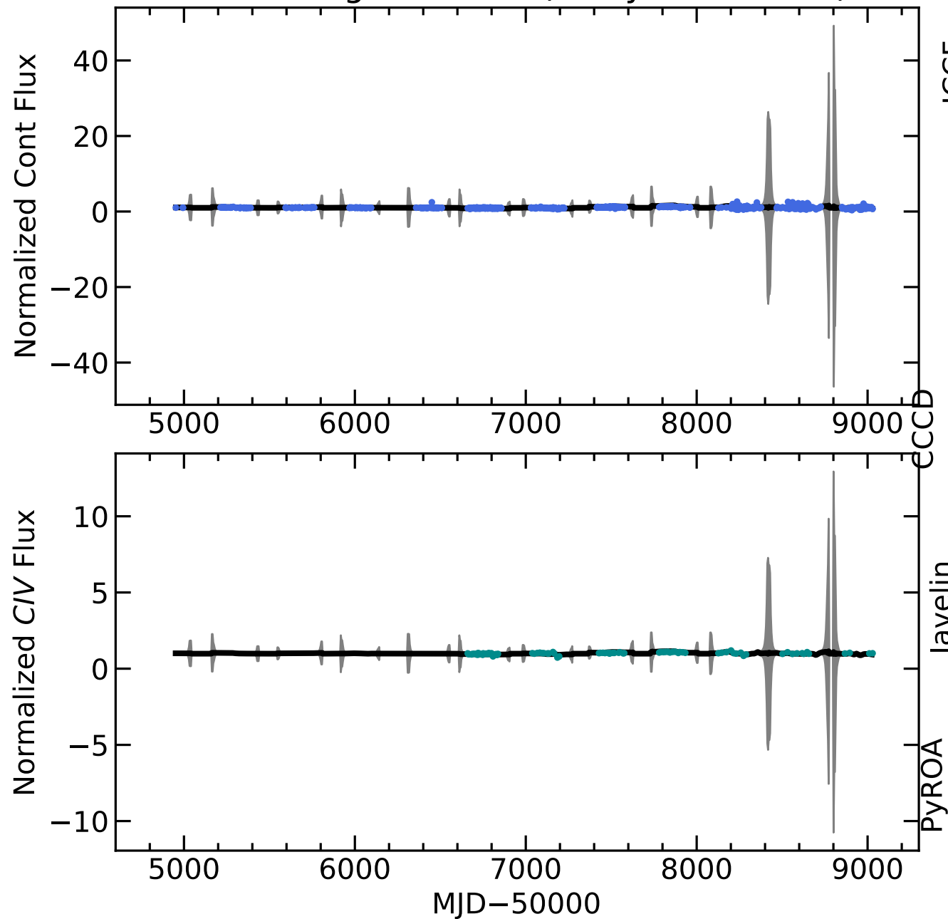
RM794 Light Curves (w/ PyROA model)
