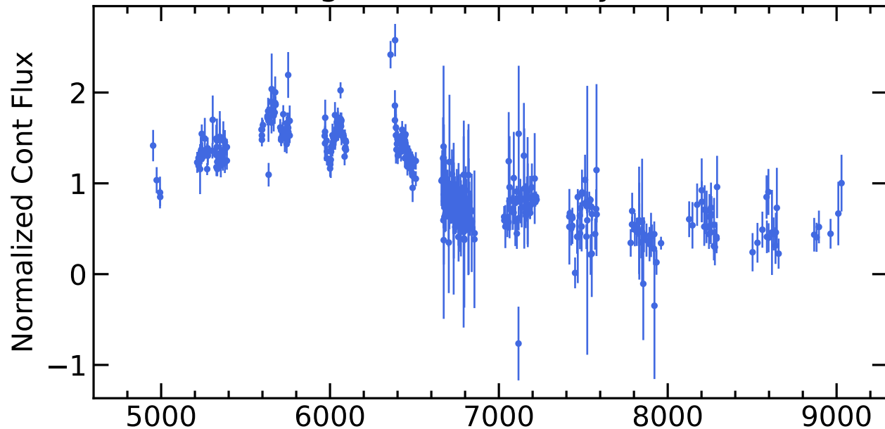
RM795 Light Curves (w/ PyROA model)
