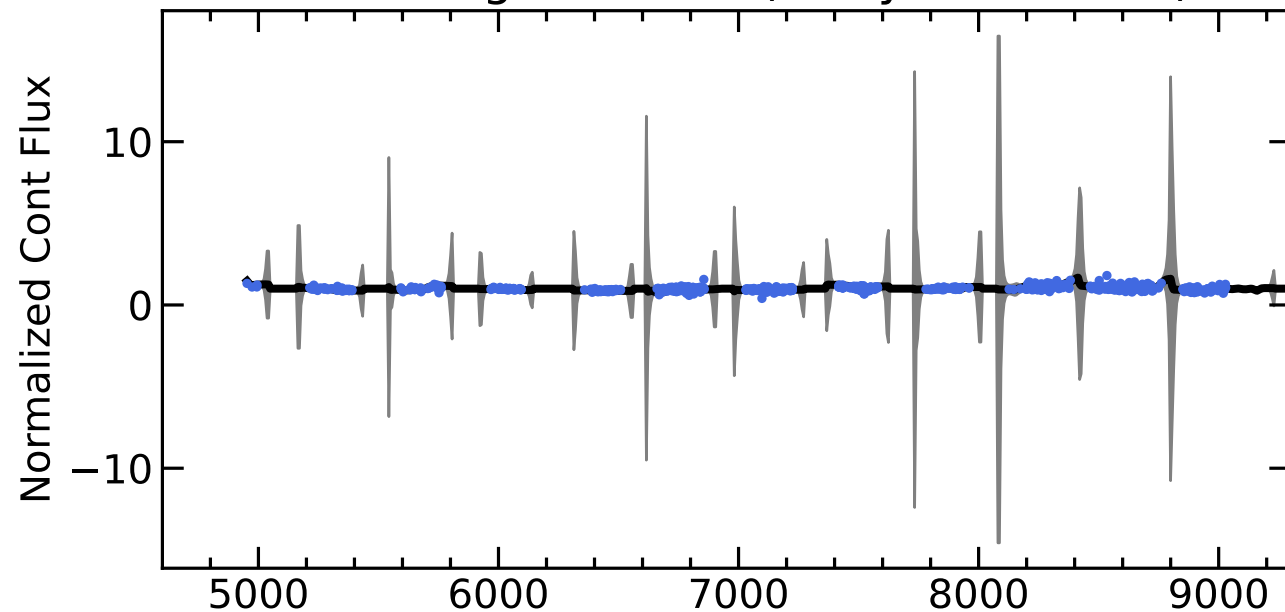
RM796 Light Curves (w/ PyROA model)
