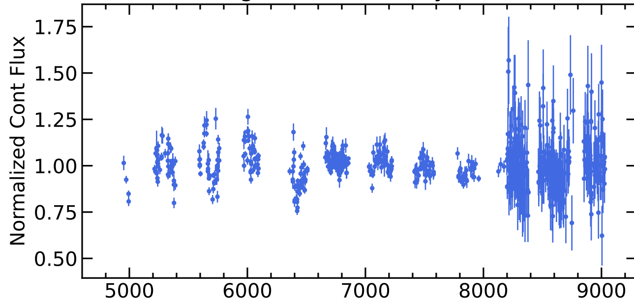
RM797 Light Curves (w/ PyROA model)
