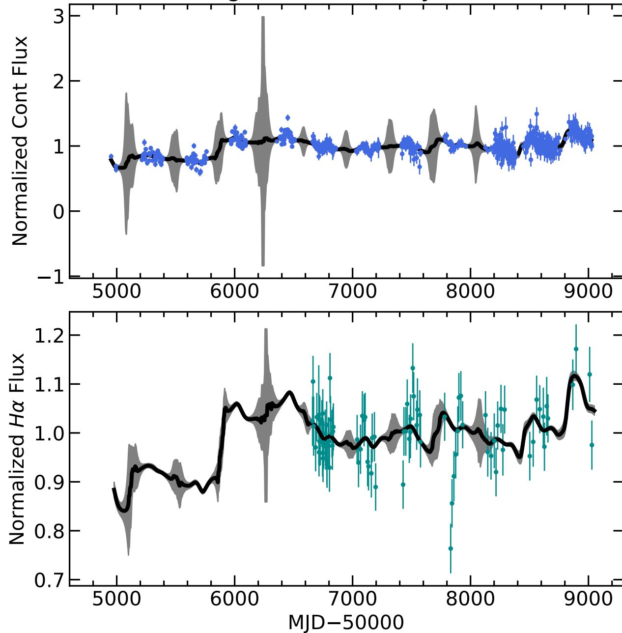
RM798 Light Curves (w/ PyROA model)
