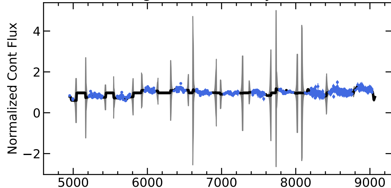
RM798 Light Curves (w/ PyROA model)
