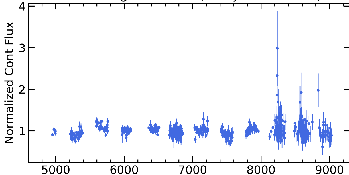
RM799 Light Curves (w/ PyROA model)
