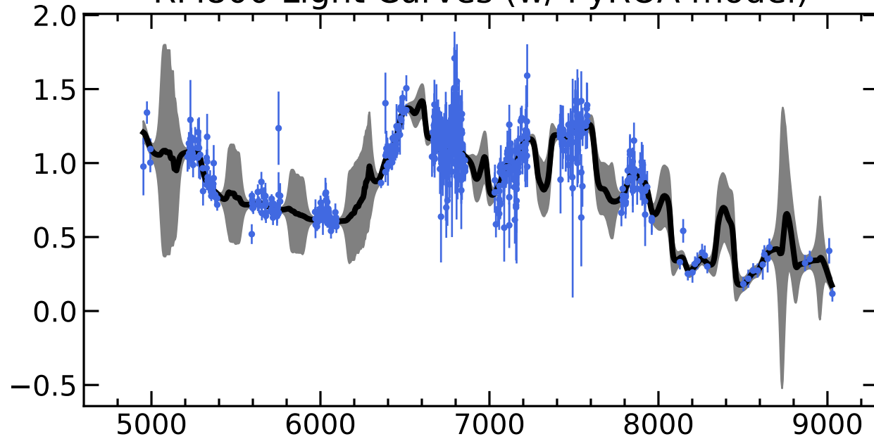
RM800 Light Curves (w/ PyROA model)
