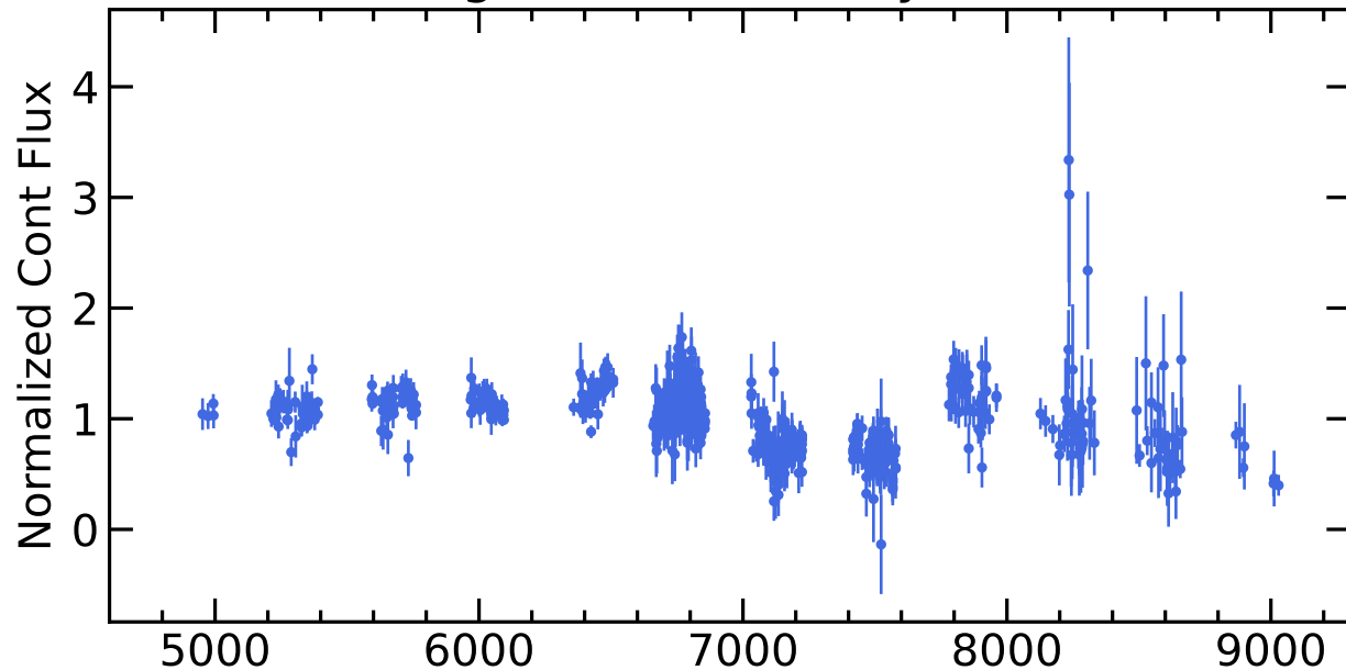
RM802 Light Curves (w/ PyROA model)
