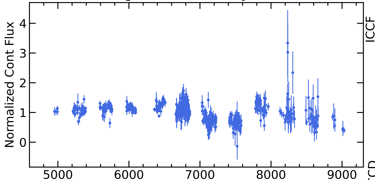
RM802 Light Curves (w/ PyROA model)
