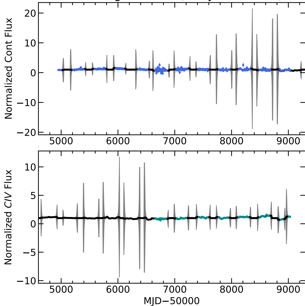
RM803 Light Curves (w/ PyROA model)
