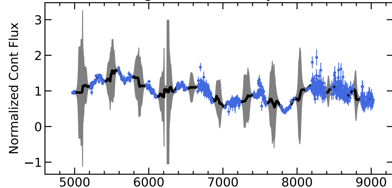
RM805 Light Curves (w/ PyROA model)
