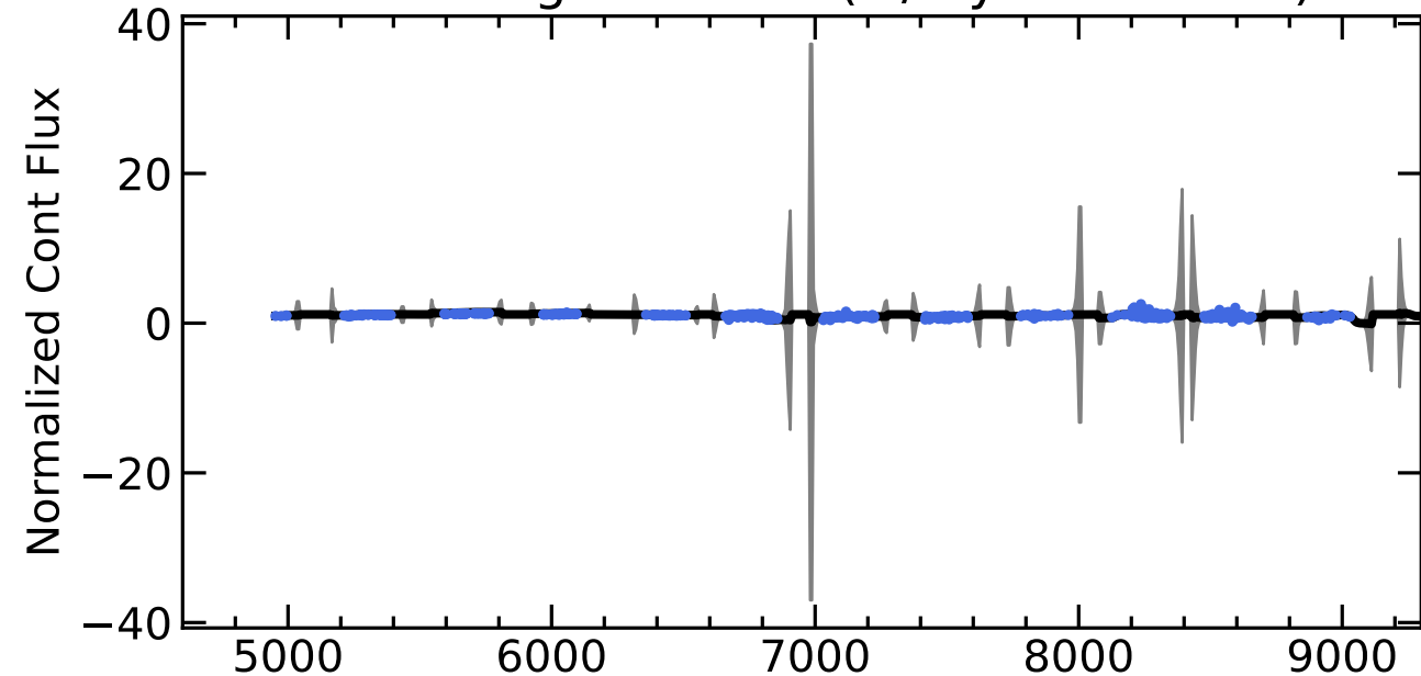
RM806 Light Curves (w/ PyROA model)
