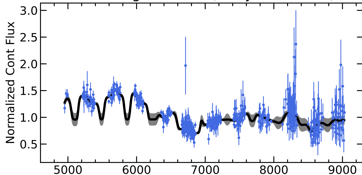
RM807 Light Curves (w/ PyROA model)
