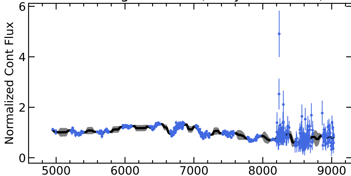
RM808 Light Curves (w/ PyROA model)
