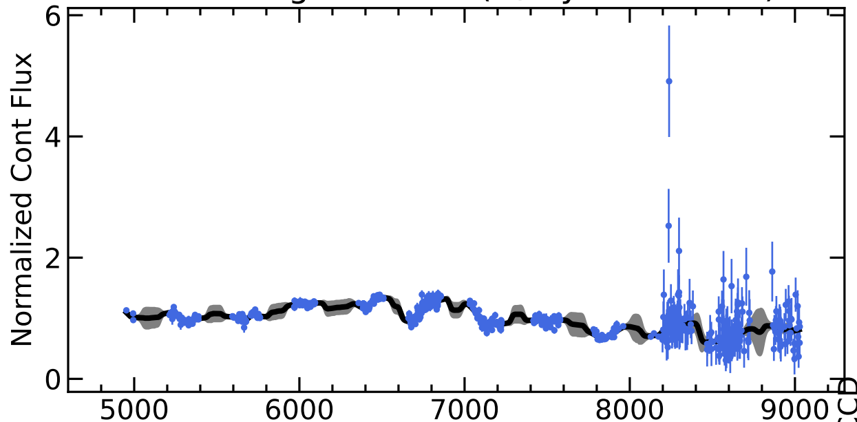
RM808 Light Curves (w/ PyROA model)
