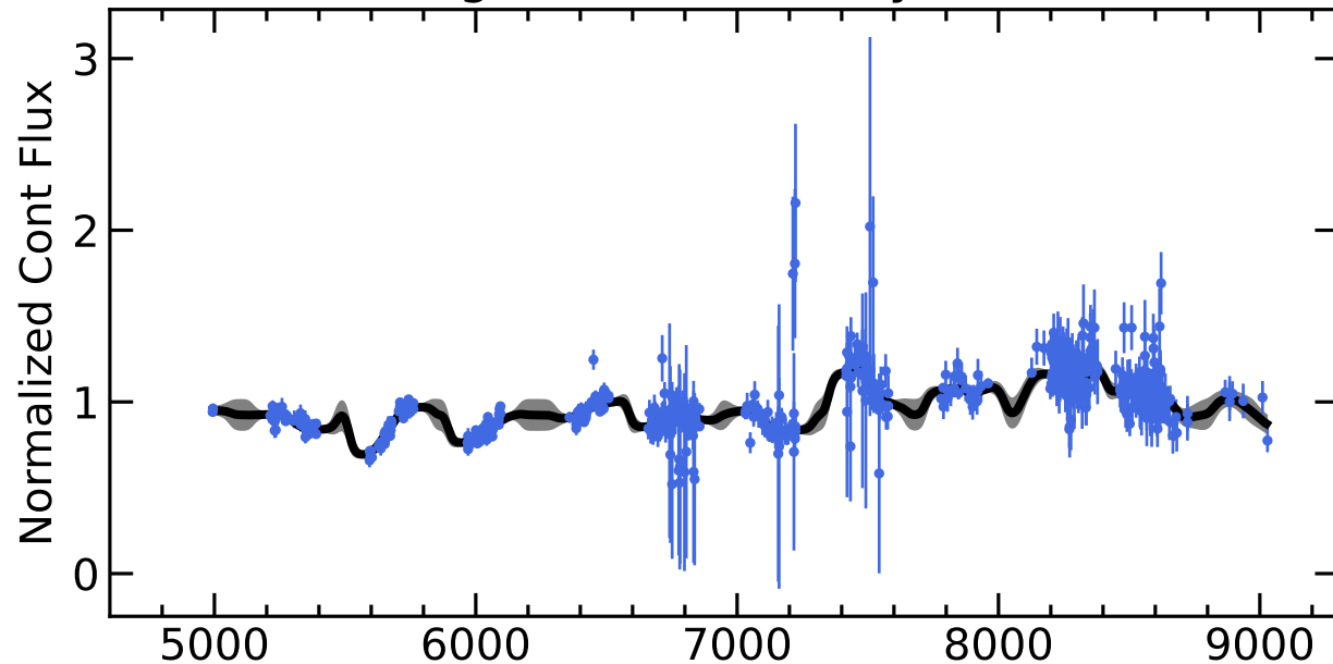
RM810 Light Curves (w/ PyROA model)
