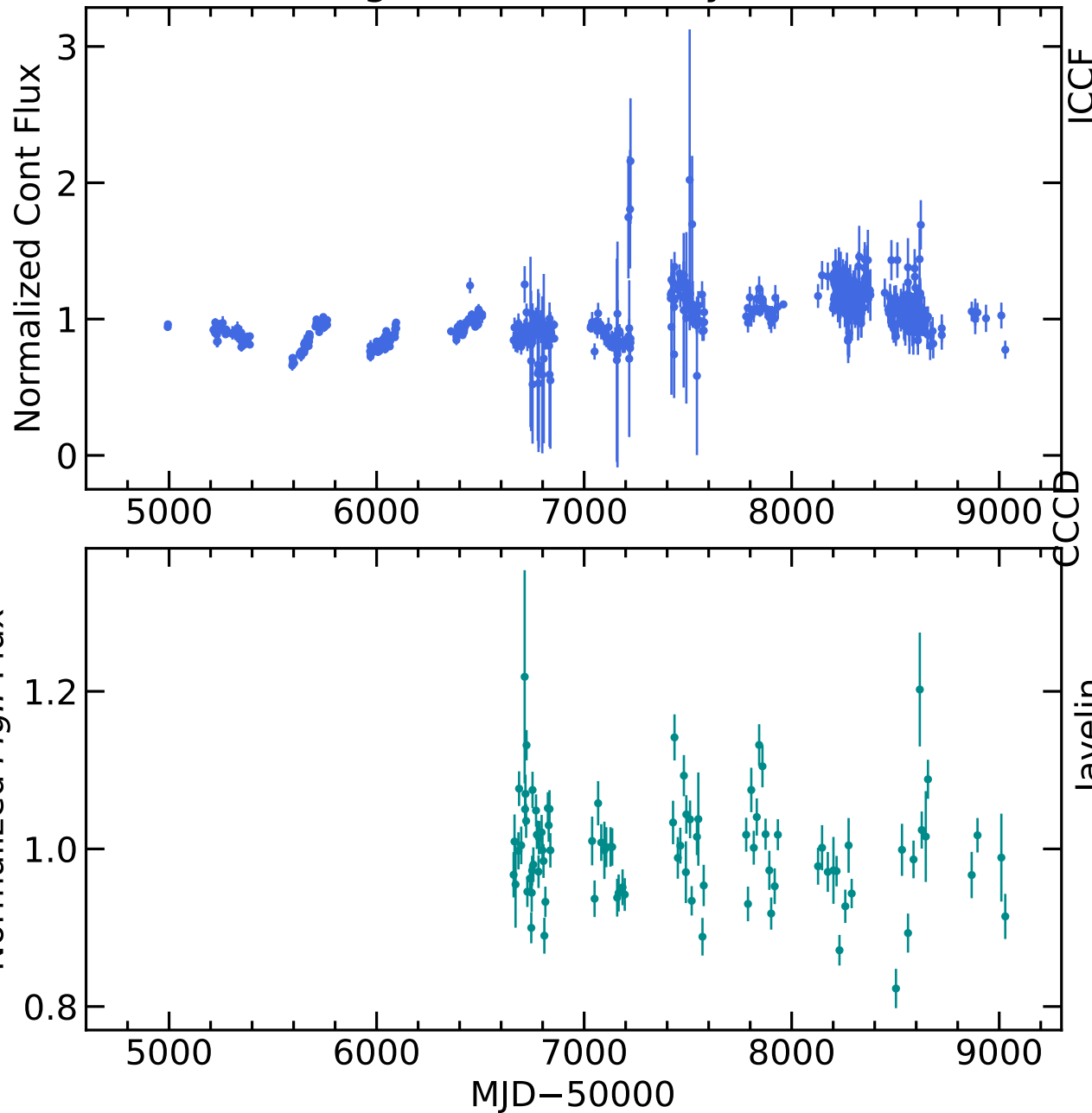
RM810 Light Curves (w/ PyROA model)
