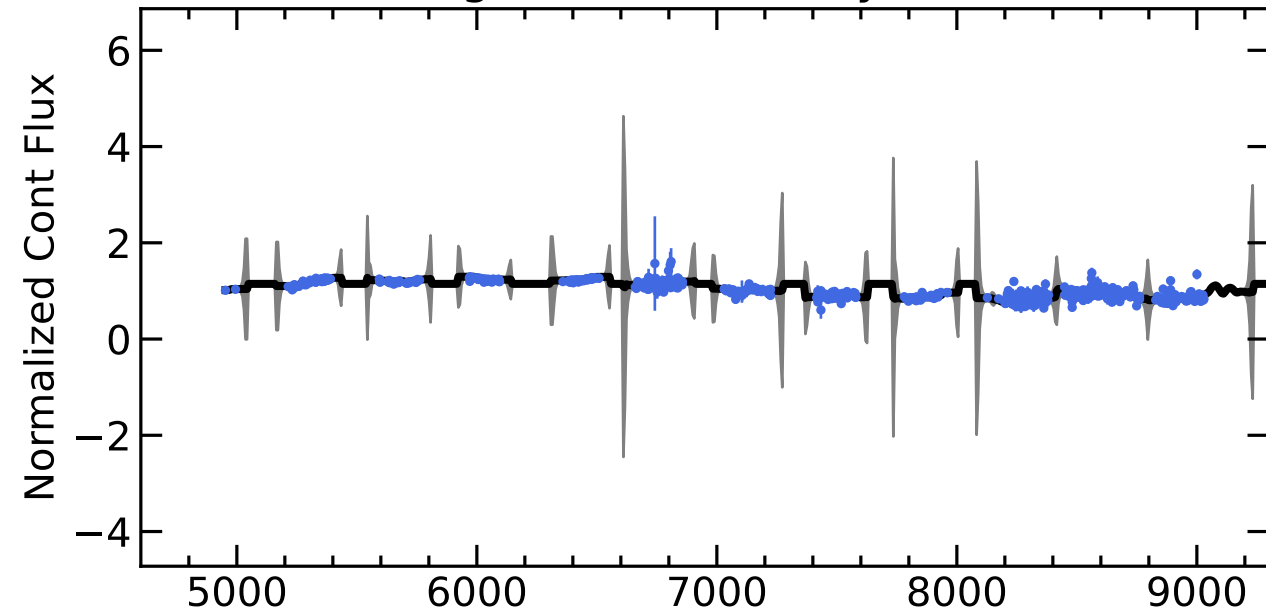
RM811 Light Curves (w/ PyROA model)
