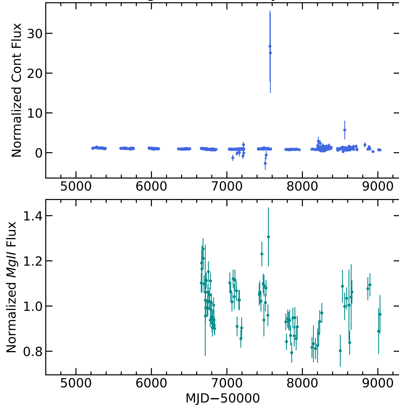
RM812 Light Curves (w/ PyROA model)
