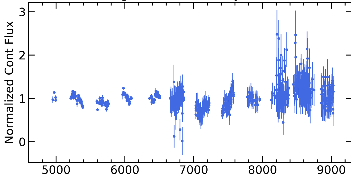
RM813 Light Curves (w/ PyROA model)
