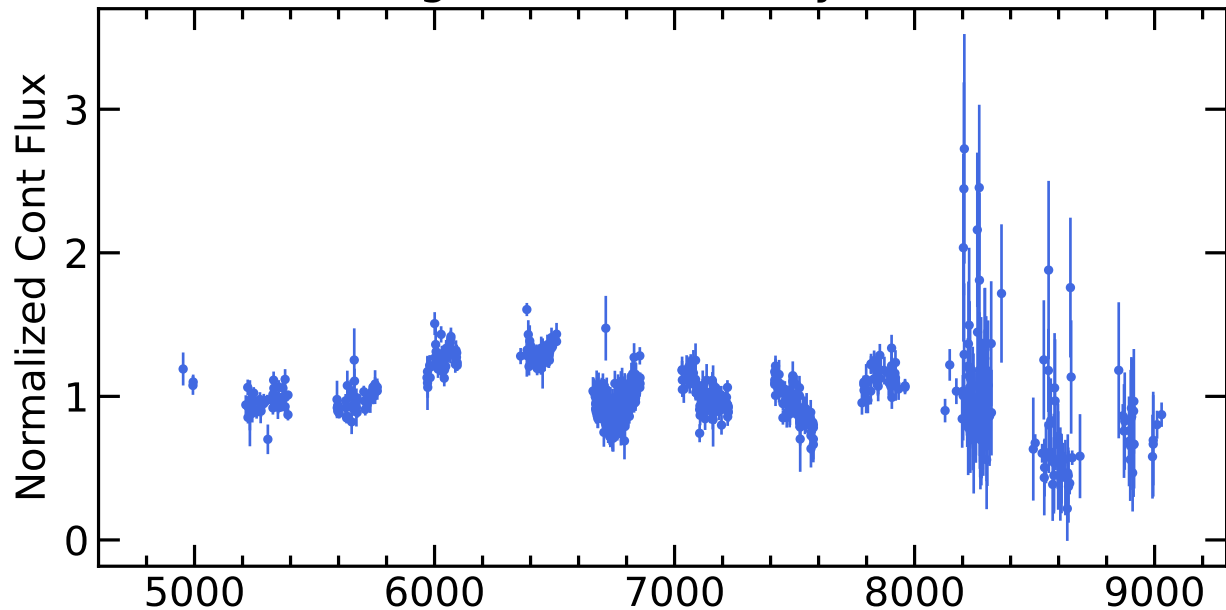
RM814 Light Curves (w/ PyROA model)
