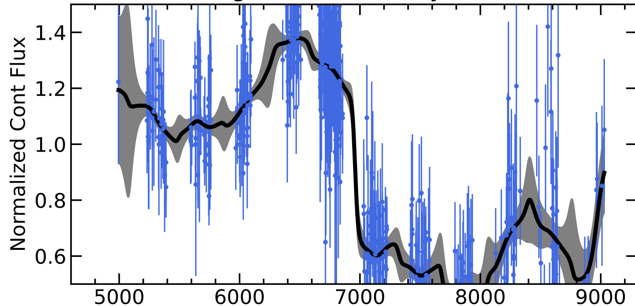
RM815 Light Curves (w/ PyROA model)
