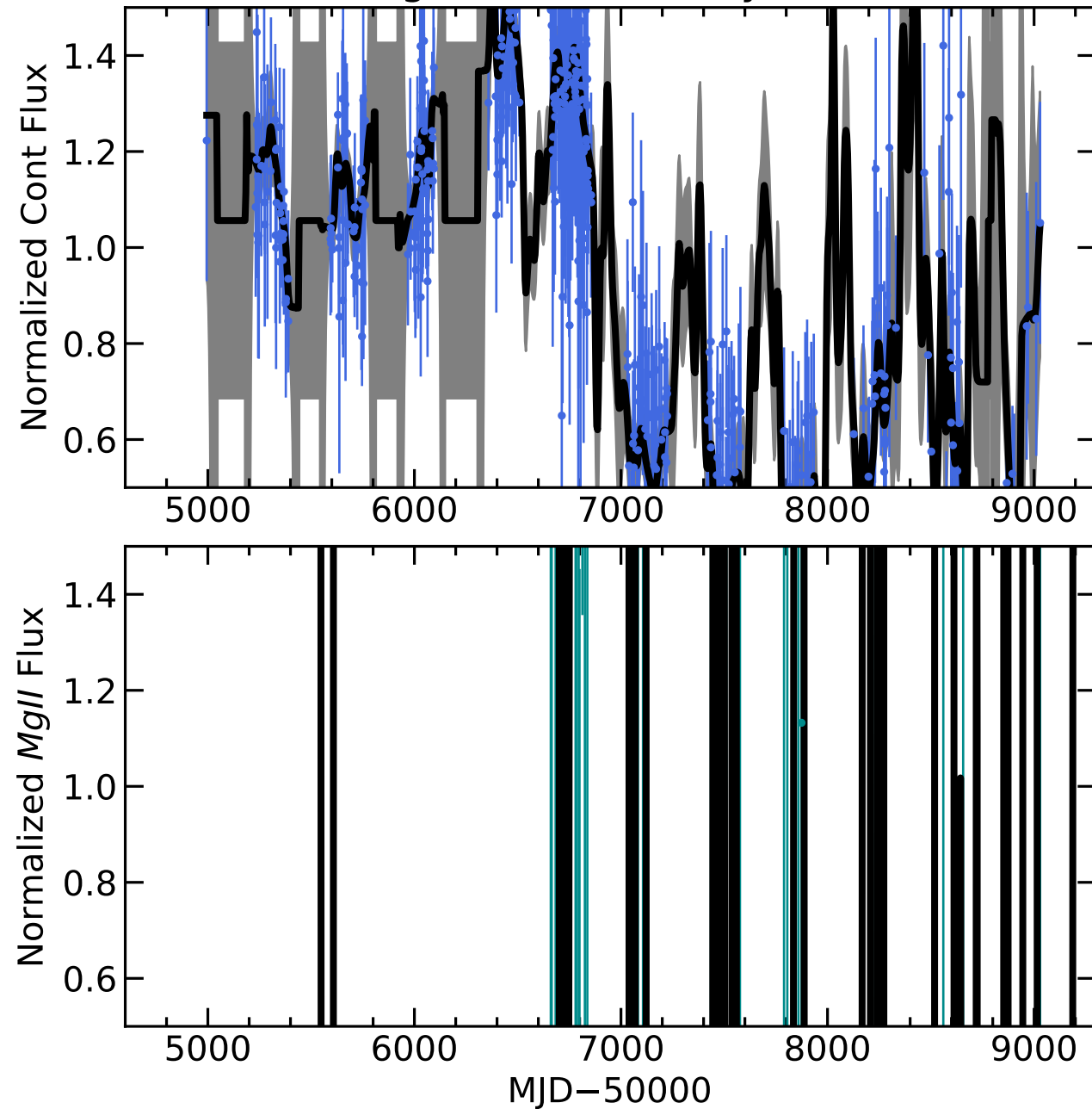
RM815 Light Curves (w/ PyROA model)
