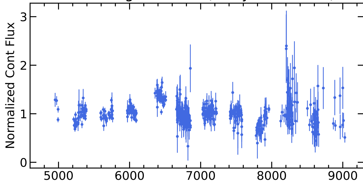
RM816 Light Curves (w/ PyROA model)
