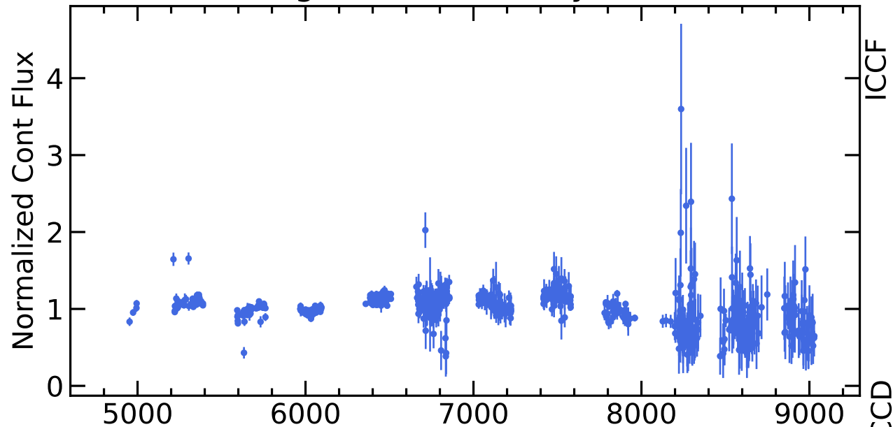
RM817 Light Curves (w/ PyROA model)
