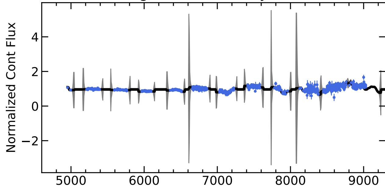
RM818 Light Curves (w/ PyROA model)
