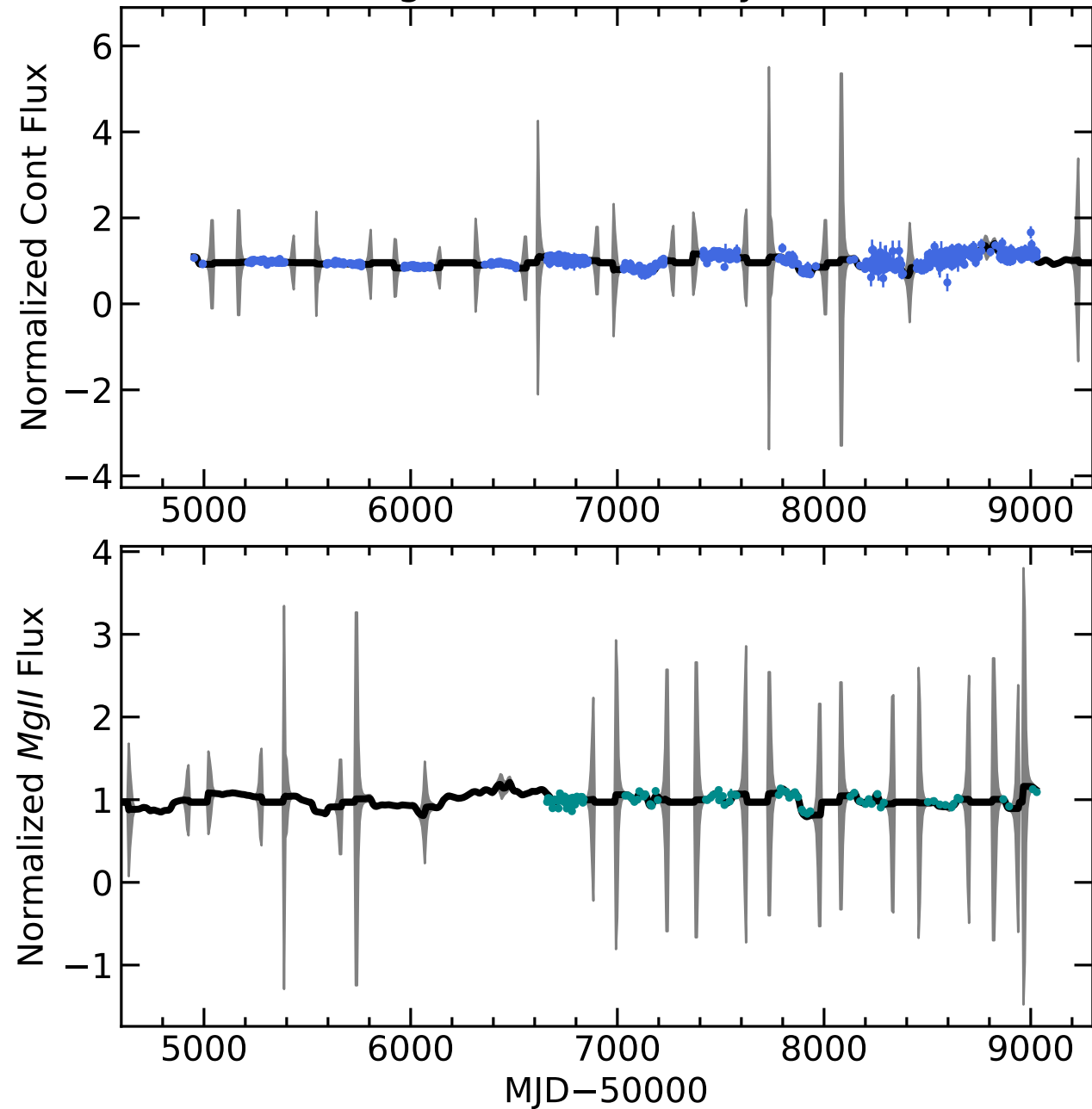
RM818 Light Curves (w/ PyROA model)
