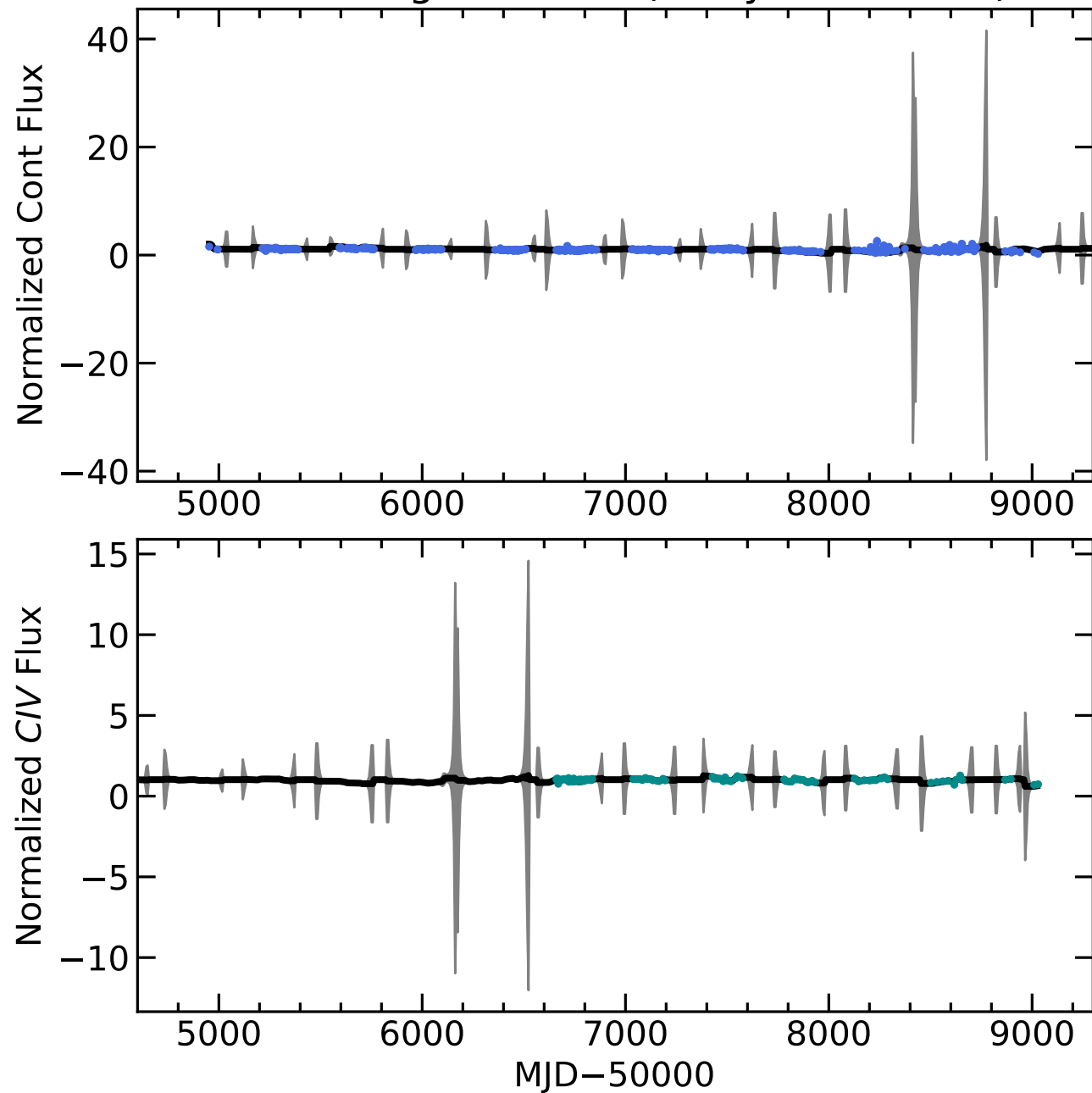
RM819 Light Curves (w/ PyROA model)
