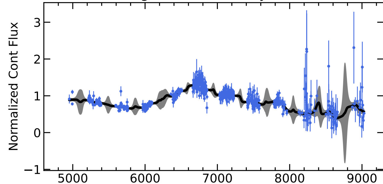
RM820 Light Curves (w/ PyROA model)
