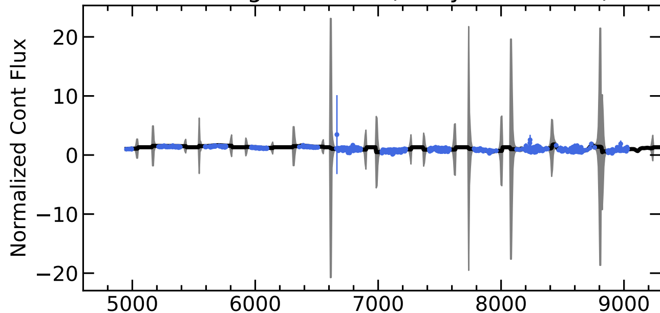
RM821 Light Curves (w/ PyROA model)
