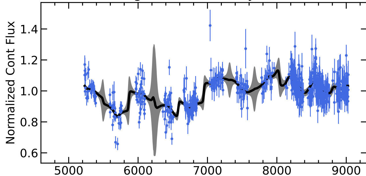
RM822 Light Curves (w/ PyROA model)
