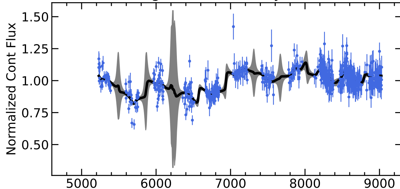
RM822 Light Curves (w/ PyROA model)
