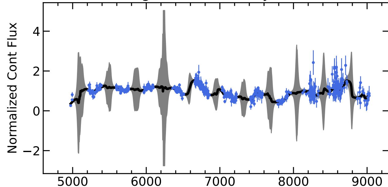
RM824 Light Curves (w/ PyROA model)
