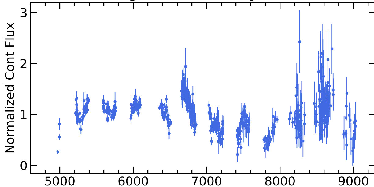
RM824 Light Curves (w/ PyROA model)
