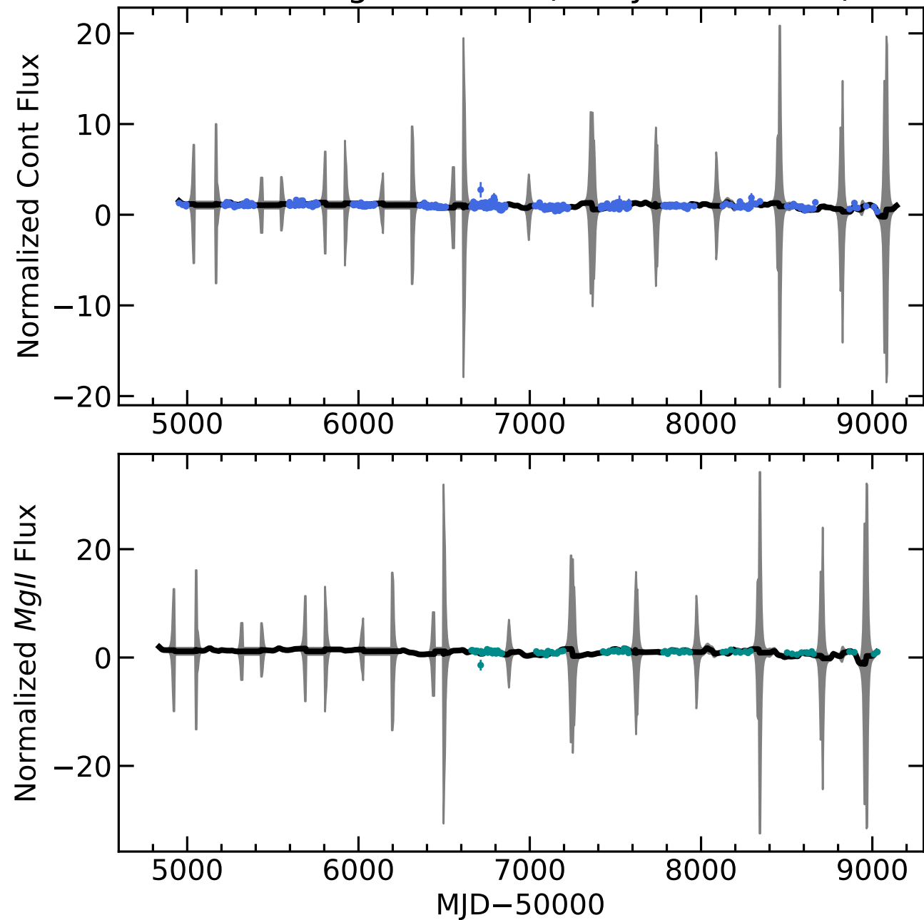
RM825 Light Curves (w/ PyROA model)
