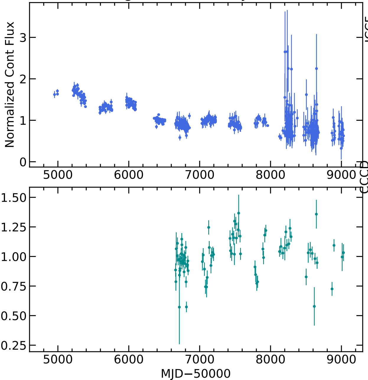
RM826 Light Curves (w/ PyROA model)
