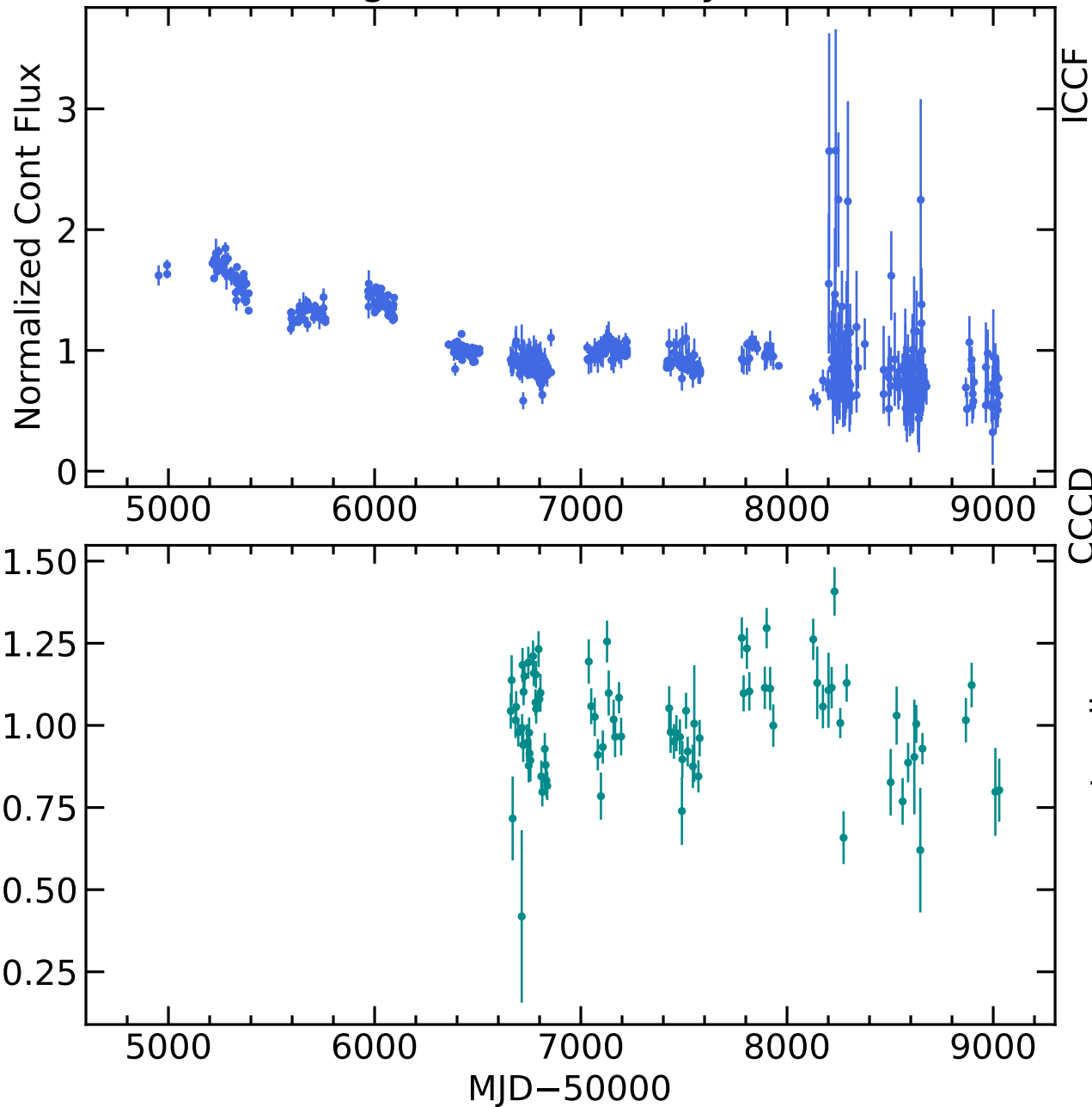
RM826 Light Curves (w/ PyROA model)
