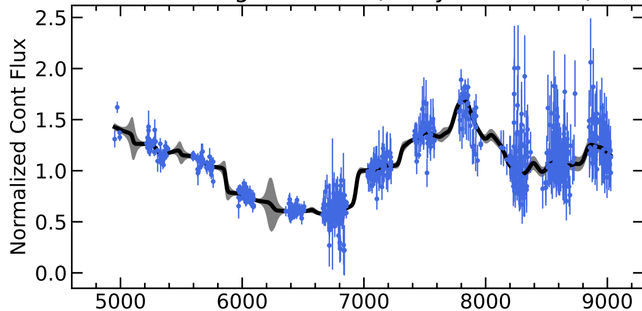
RM827 Light Curves (w/ PyROA model)
