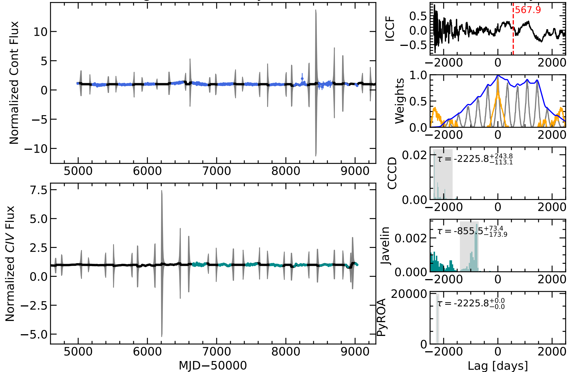
RM828 Light Curves (w/ PyROA model)
