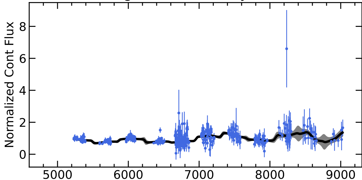
RM829 Light Curves (w/ PyROA model)
