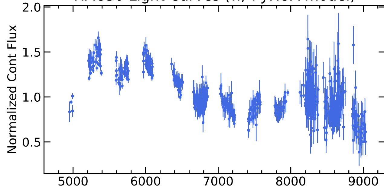
RM830 Light Curves (w/ PyROA model)
