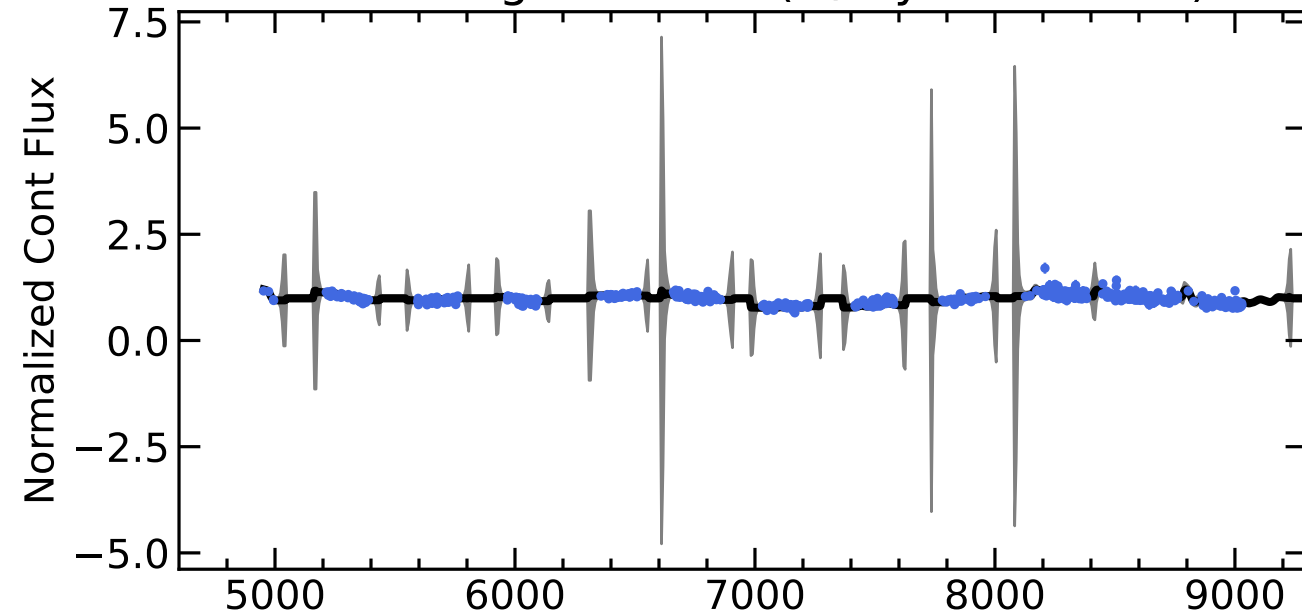
RM831 Light Curves (w/ PyROA model)
