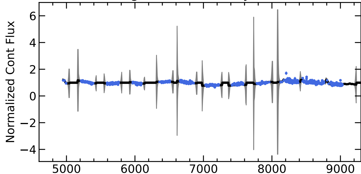
RM831 Light Curves (w/ PyROA model)
