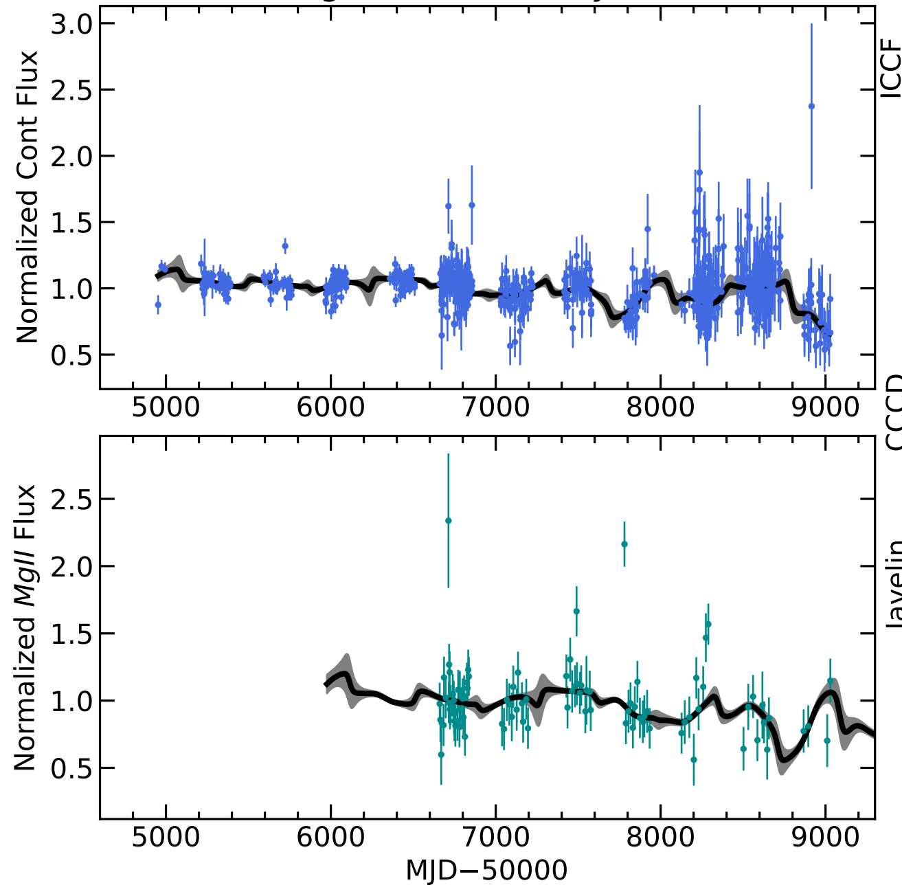
RM832 Light Curves (w/ PyROA model)
