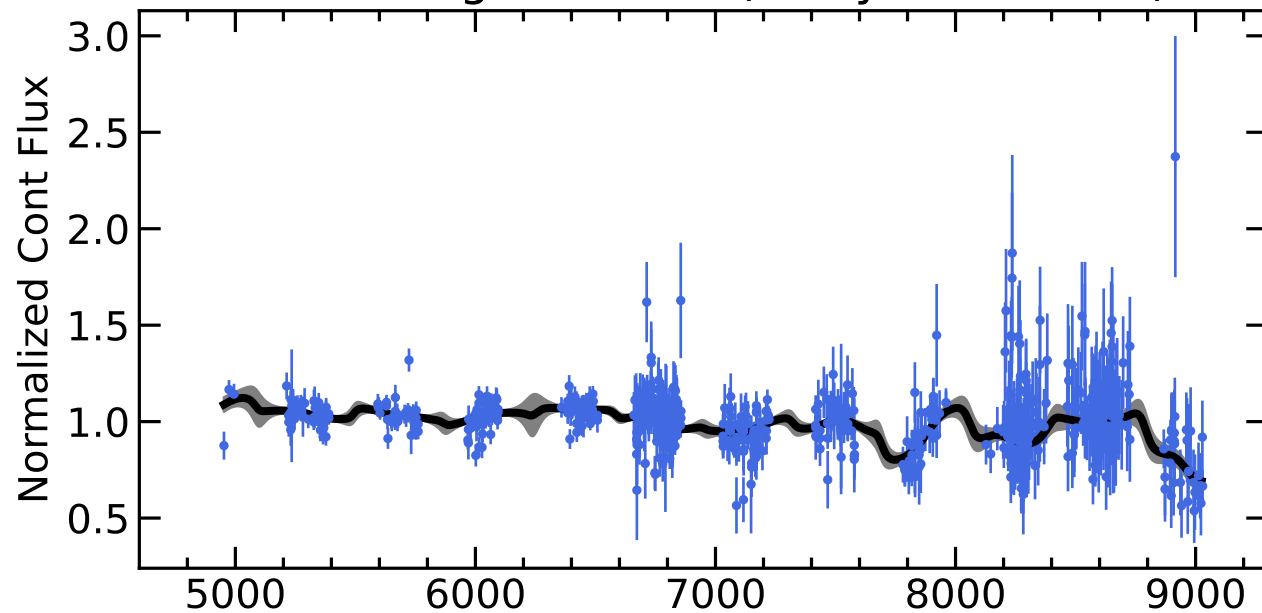
RM832 Light Curves (w/ PyROA model)
