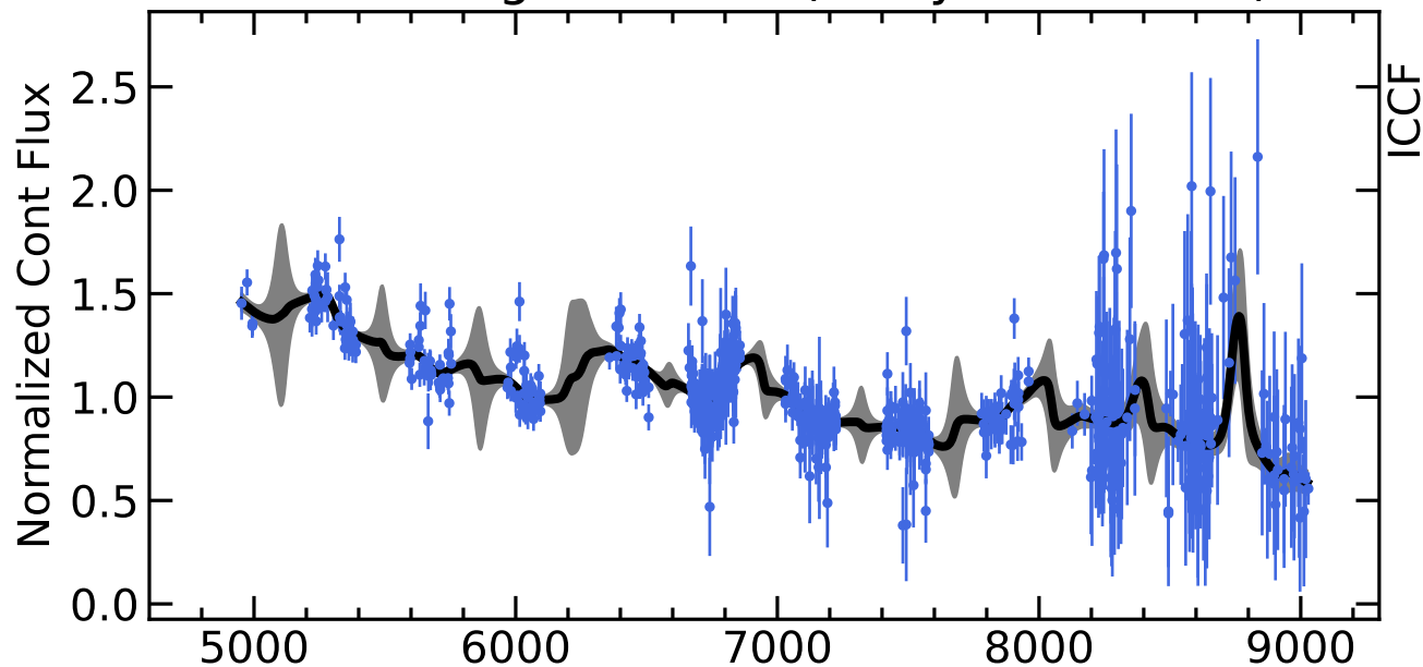
RM834 Light Curves (w/ PyROA model)
