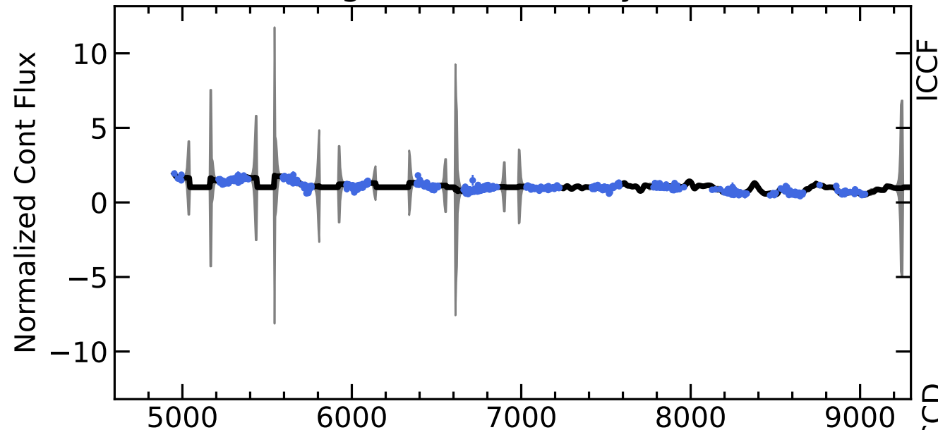
RM835 Light Curves (w/ PyROA model)
