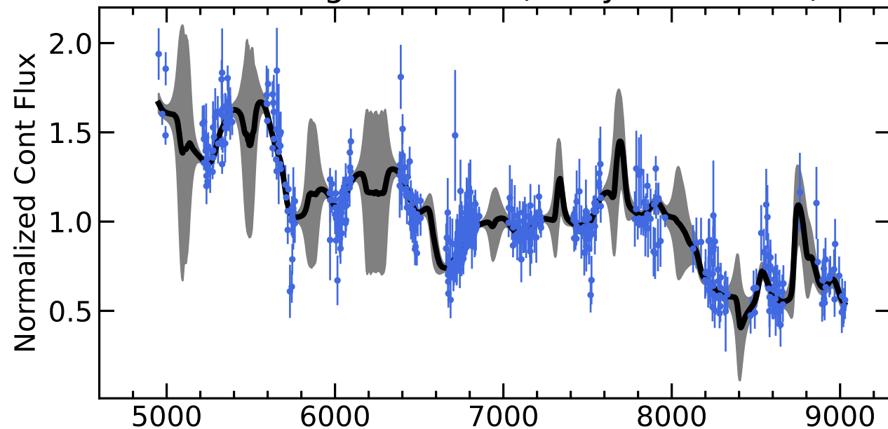
RM835 Light Curves (w/ PyROA model)
