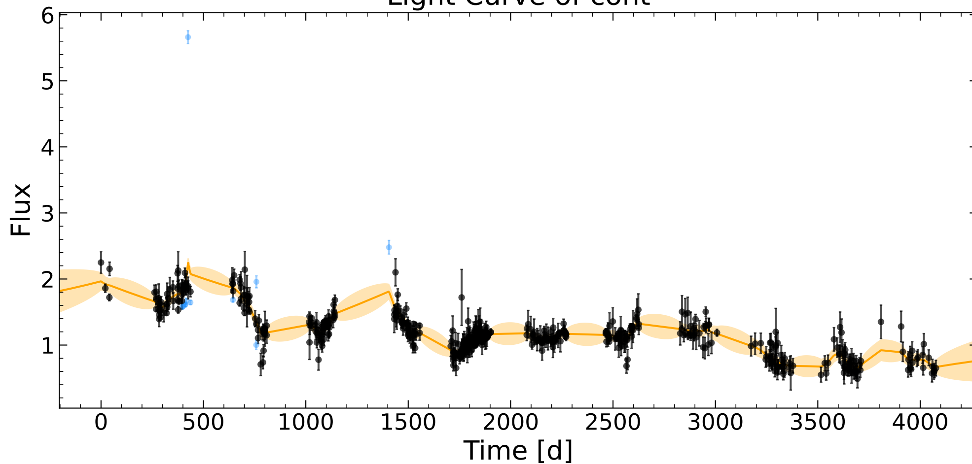
Light Curve of cont
