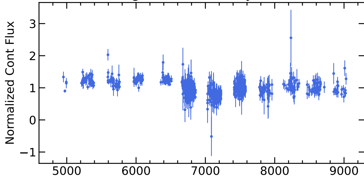
RM836 Light Curves (w/ PyROA model)
