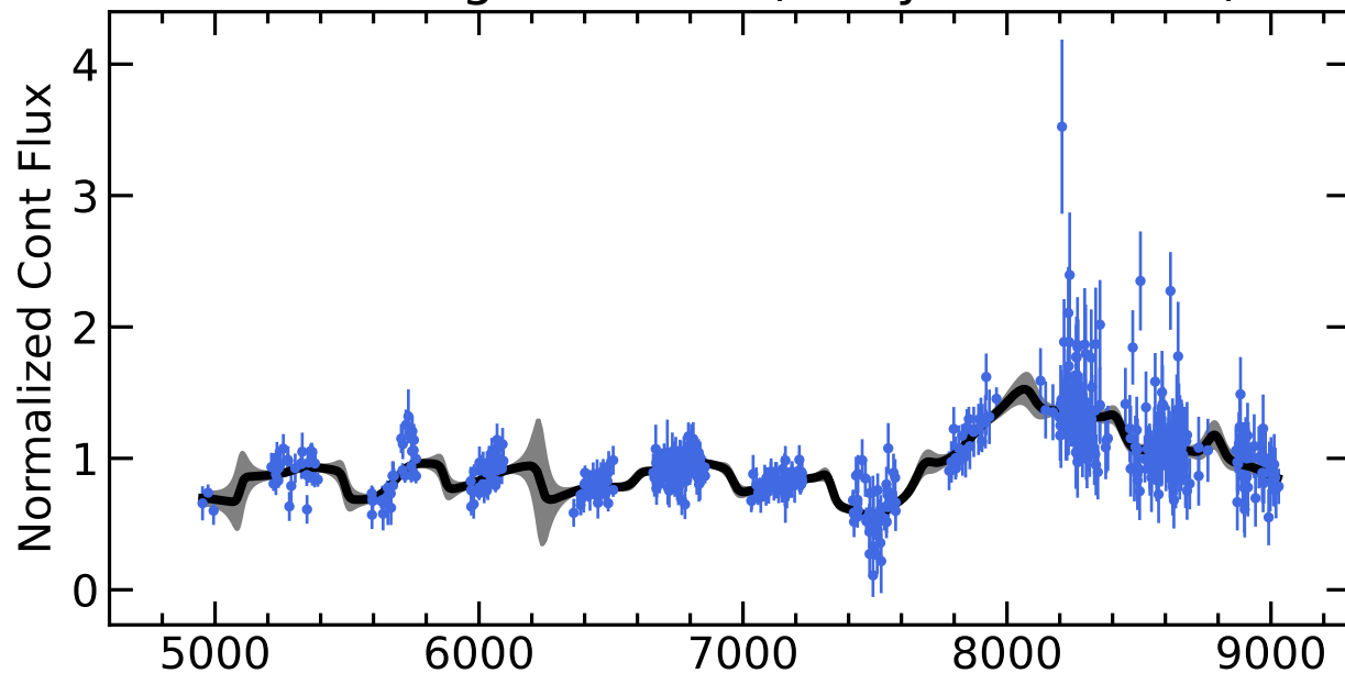
RM837 Light Curves (w/ PyROA model)
