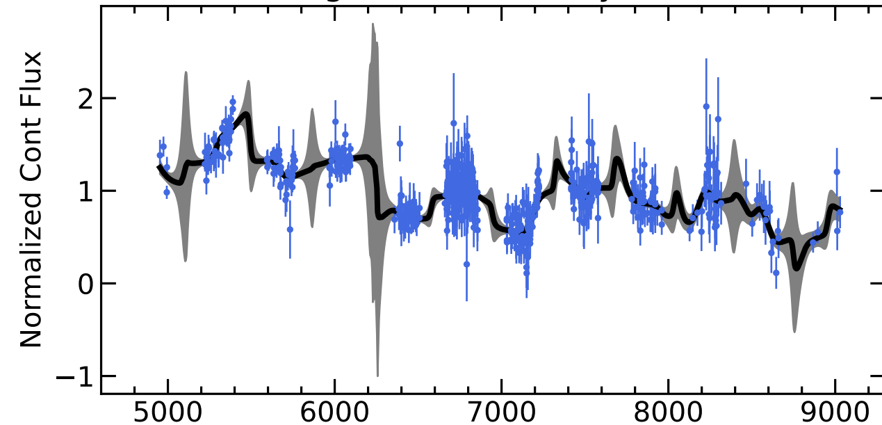
RM838 Light Curves (w/ PyROA model)
