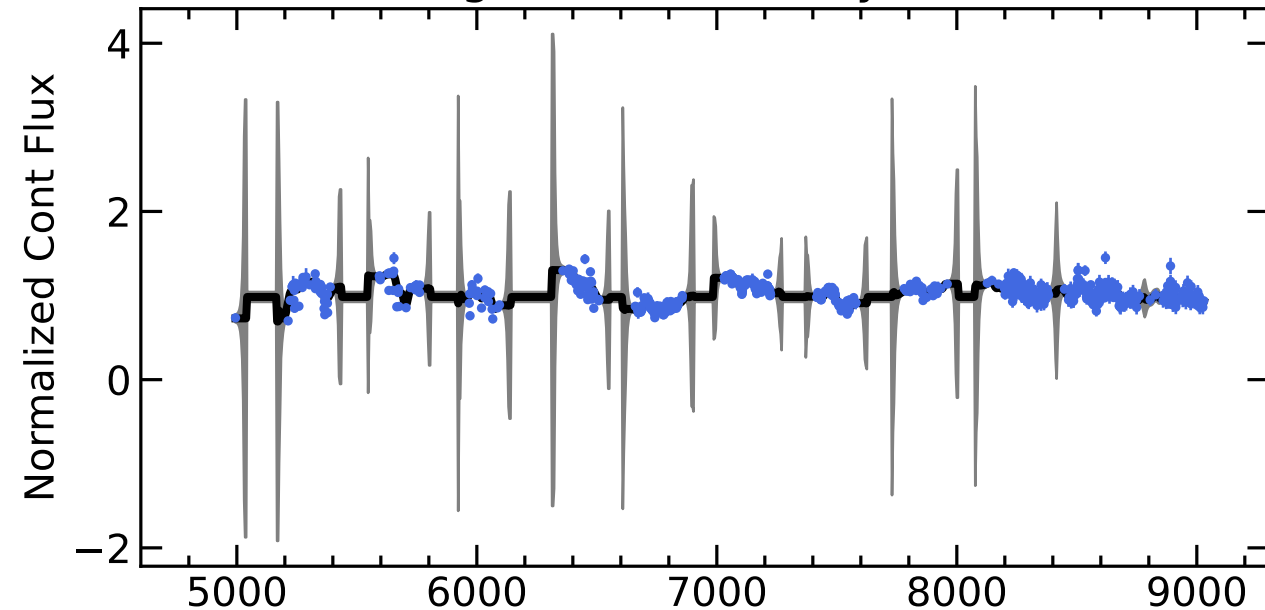
RM840 Light Curves (w/ PyROA model)
