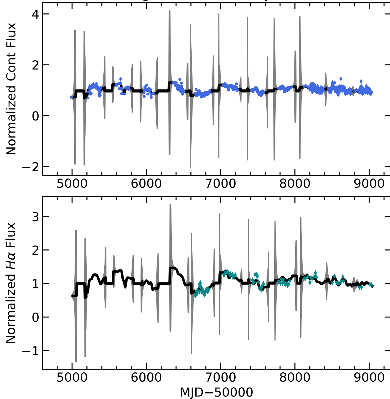
RM840 Light Curves (w/ PyROA model)
