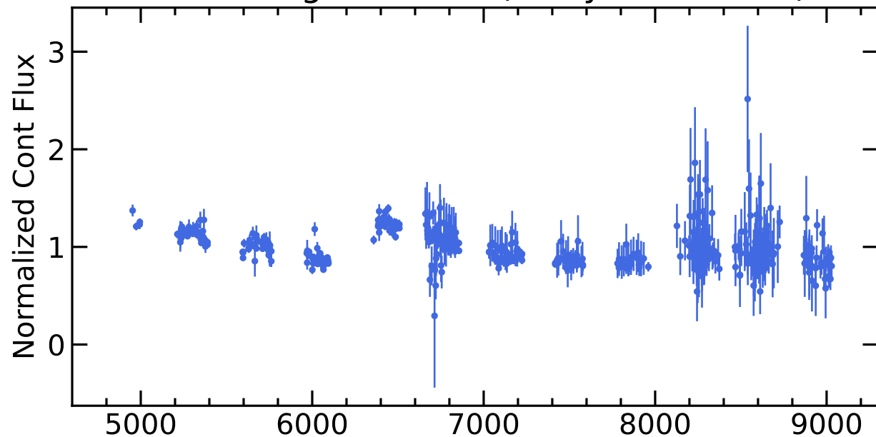
RM841 Light Curves (w/ PyROA model)
