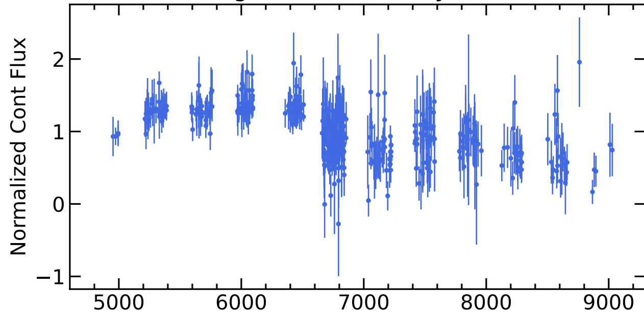
RM842 Light Curves (w/ PyROA model)
