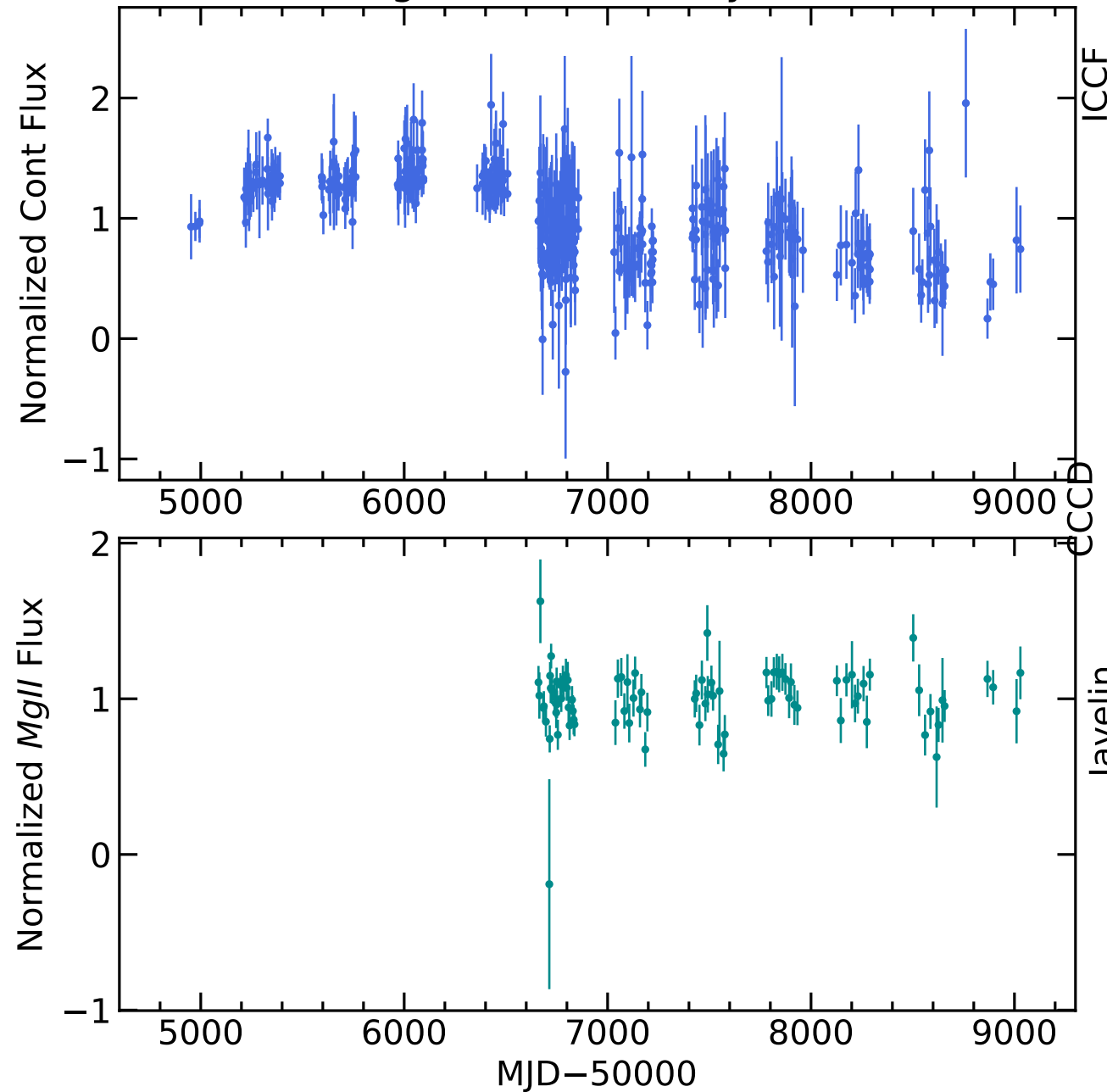
RM842 Light Curves (w/ PyROA model)
