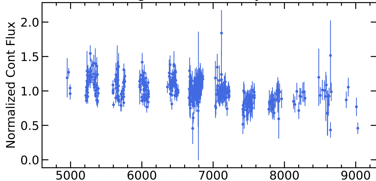
RM843 Light Curves (w/ PyROA model)
