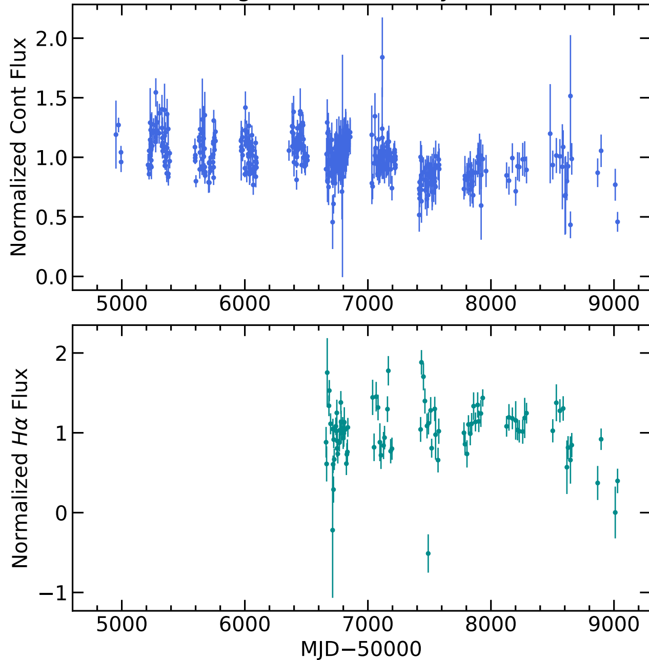
RM843 Light Curves (w/ PyROA model)
