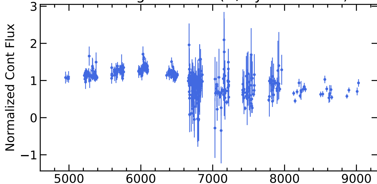
RM844 Light Curves (w/ PyROA model)
