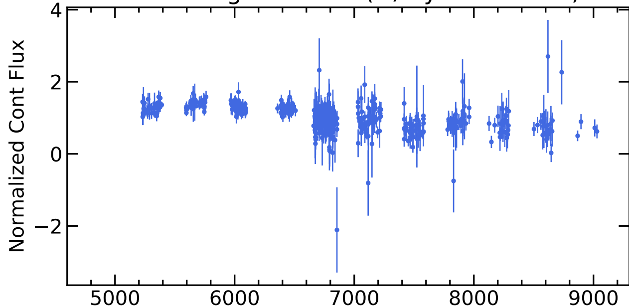
RM846 Light Curves (w/ PyROA model)
