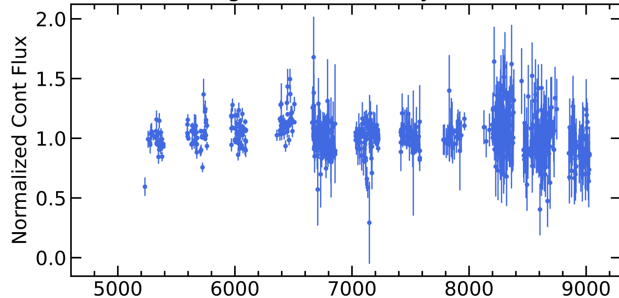
RM847 Light Curves (w/ PyROA model)
